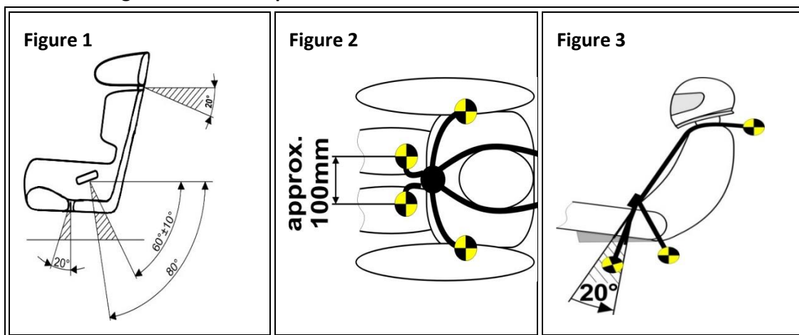
The figure above is the preferred method for harness attachment to harness bar.
